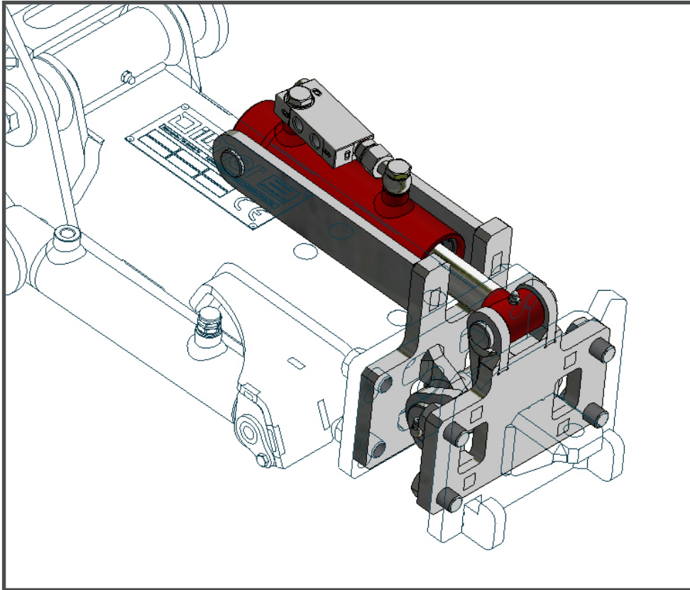
Hydraulic tilt joint for adjustable inclination of the working angle \pm 20^\circ
